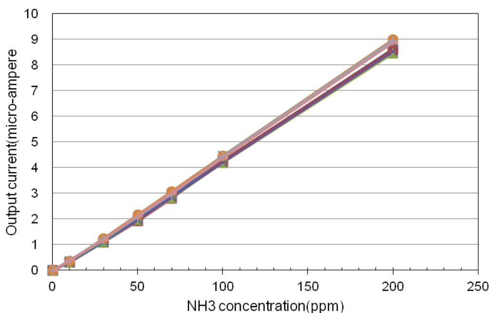
Linearity characteristics of NT-NH3-PL300 (25°C)
