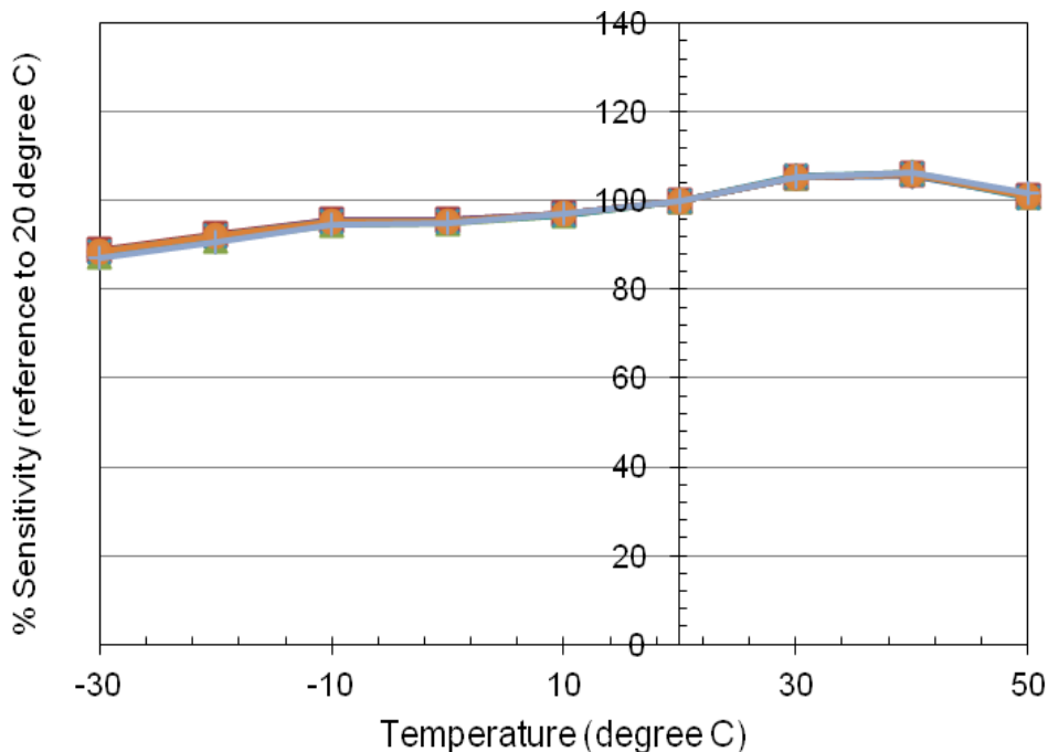
Temperature dependency of NT-NH3-PL100
