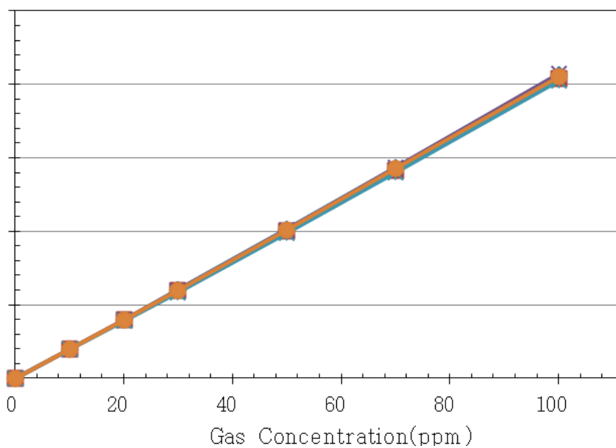
Linearity characteristics of NT-SO2-PL100 (25°C)
