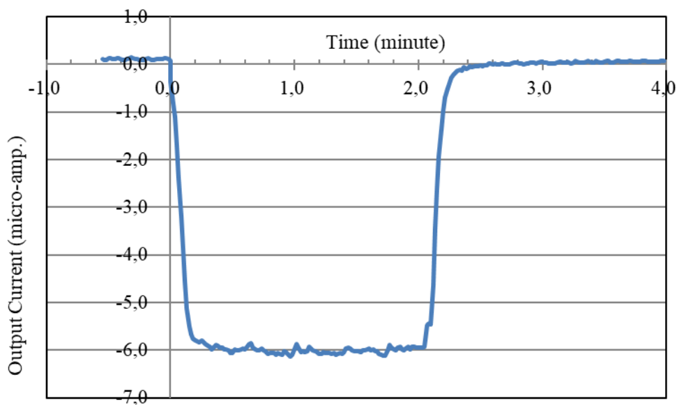
Response and Recovery characteristics of NT-NO2-PL30 (NO2:10ppm, 25°C)
