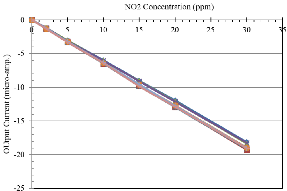
Linearity characteristics of NT-NO2-PL30 (20°C)
