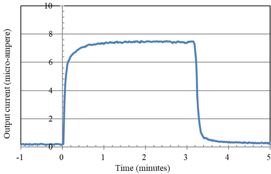
Response and Recovery characteristics of NT-H2S-PL100 (H2S:10ppm, 20°C)
