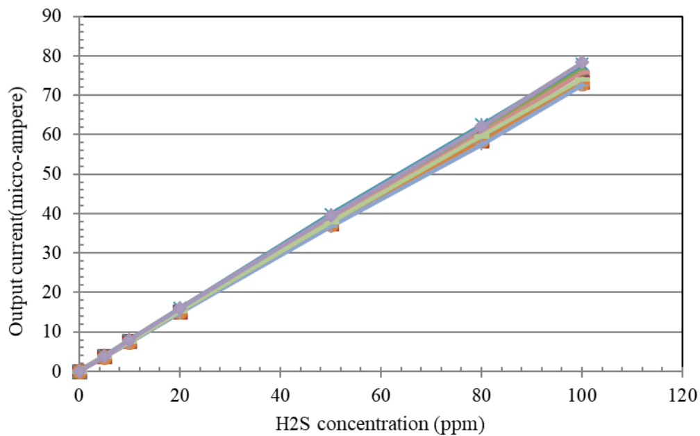
Linearity characteristics of NT-H2S-PL100 (20°C)
