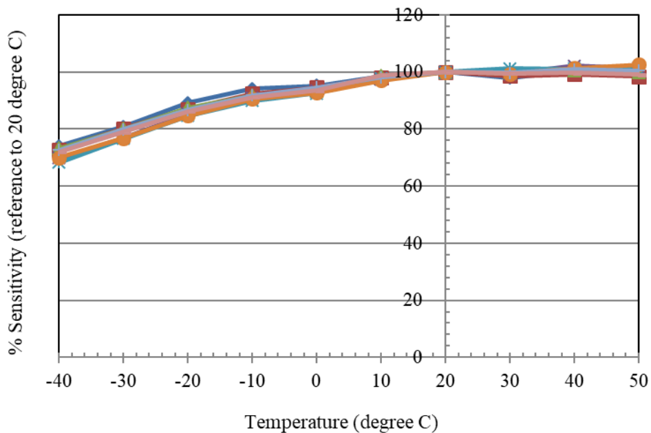
Temperature dependency of NT-H2S-PL100
