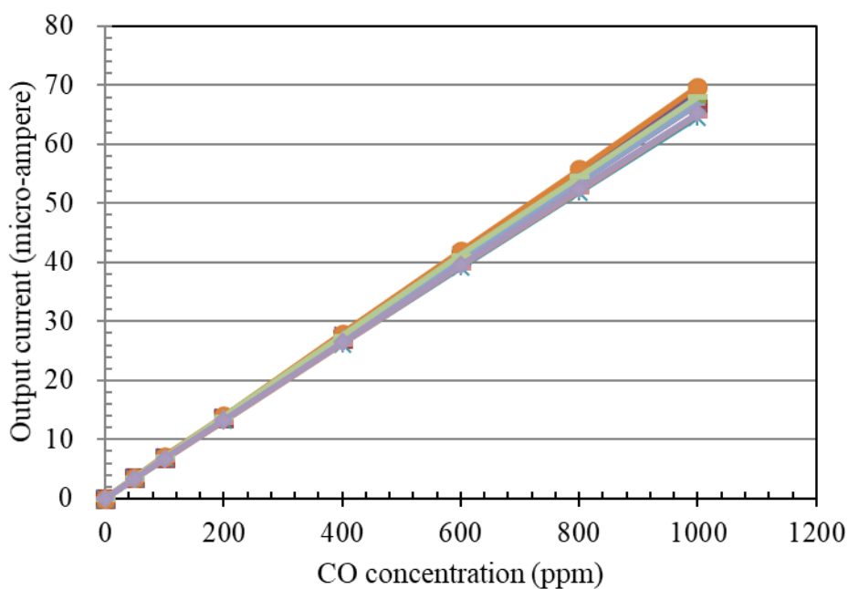
Linearity characteristics of NT-CO-PL1000 (25°C)
