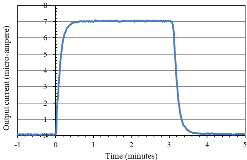
Response and Recovery characteristics of NT-CO-PL1000 (CO:100ppm, 20°C)
