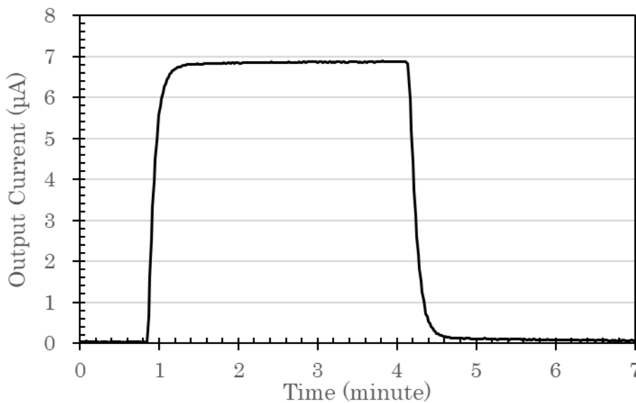
Response and Recovery characteristics of NT-CO-PL2000-HT (CO:100ppm, 20°C)
