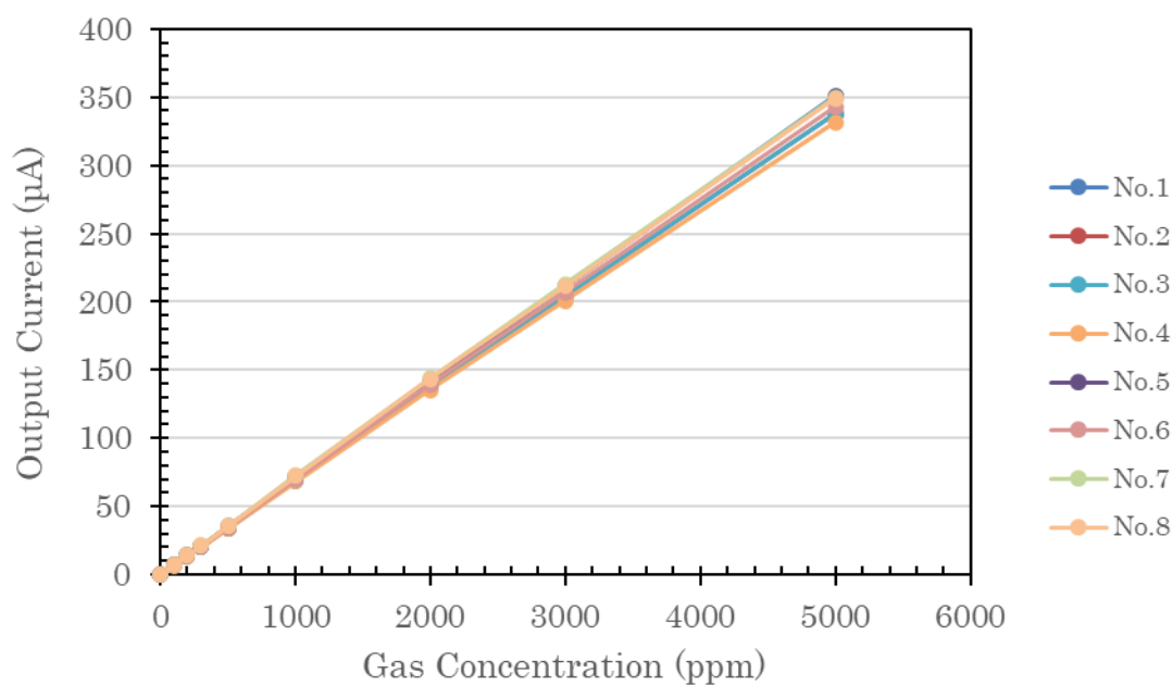
Linearity characteristics of NT-CO-PL2000-HT (25°C)
